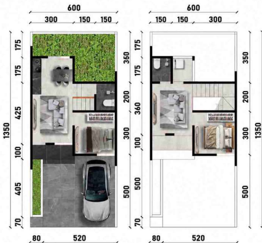
Lantai 1
