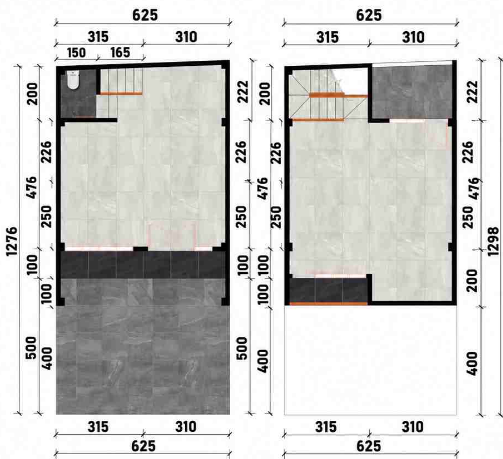
Lantai 1
